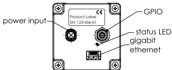
Figure 2: Rear of StarForm-Swift with replacement M12 connectors
