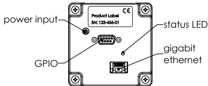
Figure 1: Rear of StarForm-Swift with original connectors
